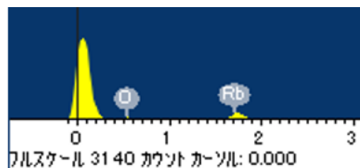
Fig. 2 EDX analysis of the thin film.
