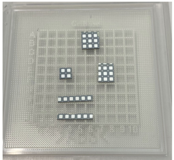
Fig. 1 Pixel diode array after cutting
