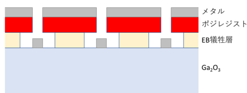
Fig. 1 Cross-sectional schematic diagram after metal deposition
