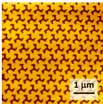
Fig.1 AFM image of chiral metamaterial made by Pt.
