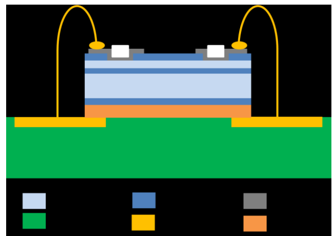
Fig. 1 Schematic illustration of ball bonding sample (cross section).
