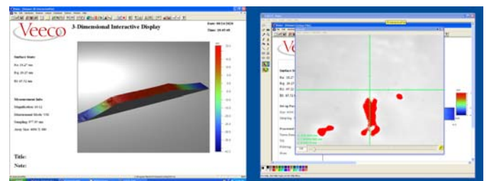
Fig. 3 Three dimension shape data of No.5 specimen
