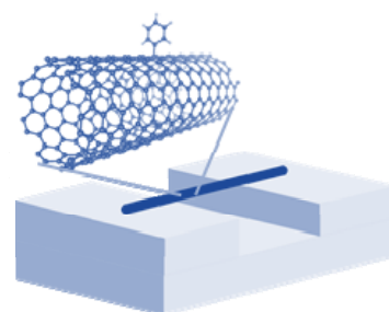
Fig. 1 Schematic of a functionalized SWNT suspended across a trench of SiO 2 /Si substrate.
