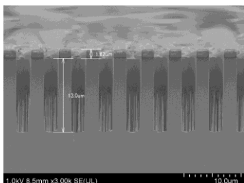
Fig. 1 SEM image of the needle like bottom structure.
