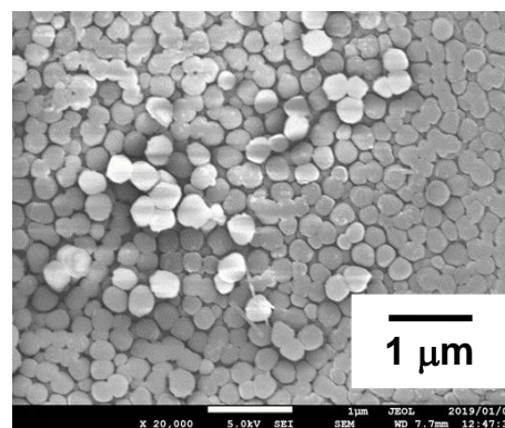
Fig. 1 SEM image of polymer pillar film obtained by nanoimprinted under 80 °C. .
