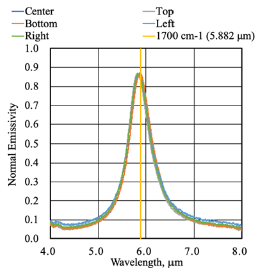
Fig. 2 Normal emissivity
