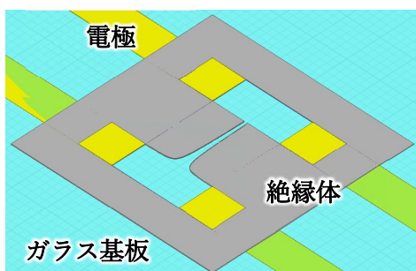
Fig. 1 Structure of Insulator-Based DEP Device
