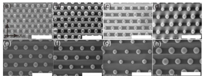
Fig. 1 Scanning electron microscopic (SEM) images of the Al nanocylinder array with the pitch p = (a) 150, (b) 180, (c) 200, (d) 220, (e) 255, (f) 275, (g) 300, and (h) 330 nm. Scale bars = 500 nm.
