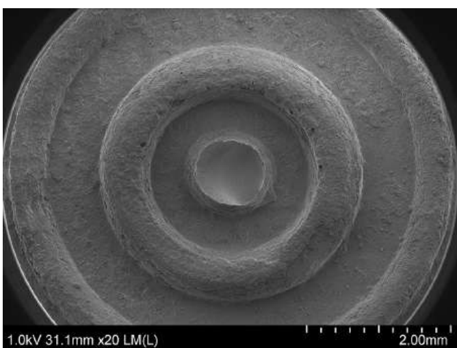
Fig. 3 SEM image of Indus seal.
