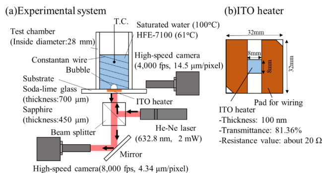
Fig. 1 Experimental apparatus
