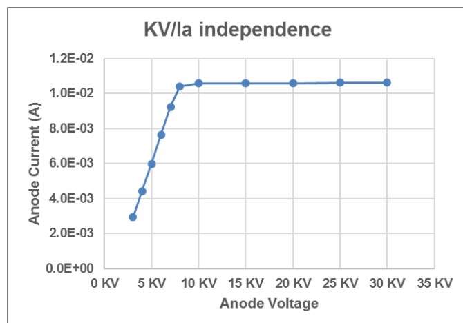
Fig. 2 KV/Ia independence
