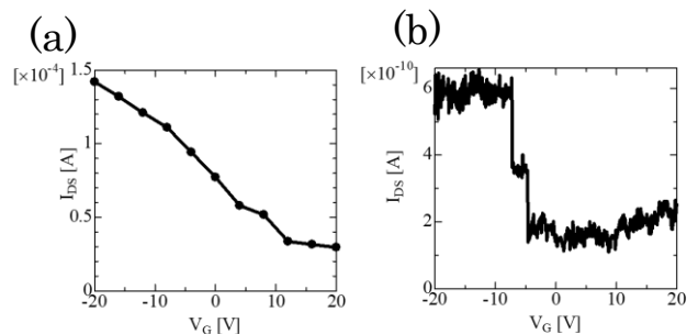
Figure 1 - Back-gate transfer characteristics of the carbon thin film FET whose channel size is 20 μm × 2 μm (width × length). The dependences of the FET characteristics on the substrate (a) Al 2 O 3 and (b) ZrO 2 when the source-drain voltage ( V_{SD} ) was 1.0 V.
