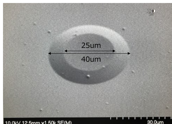
Fig. 1 SEM image of etched PZT film.
