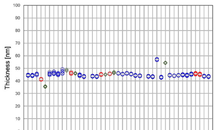
Fig. 1 Result of SiO 2 film thickness measurement.
