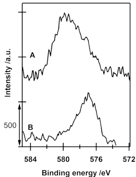
Fig. 1 Cr 2p 3/2 XPS spectra of Ce-Cr-4d mixed metal oxides.
