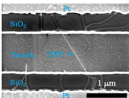
Fig. 1: SEM image of CNT field effect transistor.
