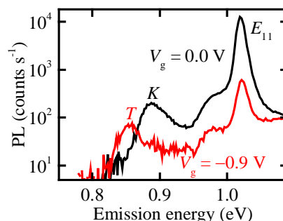
Fig. 2: Single CNT photoluminescence spectrum. At high gate voltage, the exciton peaks ( E_{11} and K ) quench and the new trion peak ( T ) appears.
