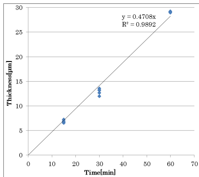
Figure 1. Ashing rate of multilayer film
