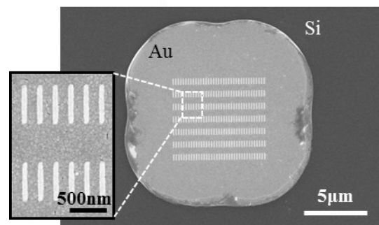
Fig. 1 SEM images of the fabricated gold nanorod array on gold thin films.
