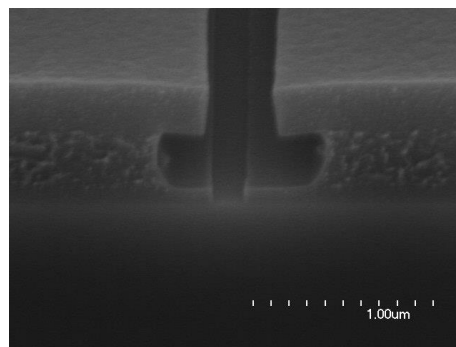
Fig. 1 Cross-sectional SEM image of developed resist pattern.
