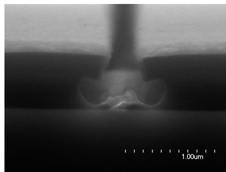
Fig. 2 Cross-sectional SEM image of Ni/Au electrode after deposition.
