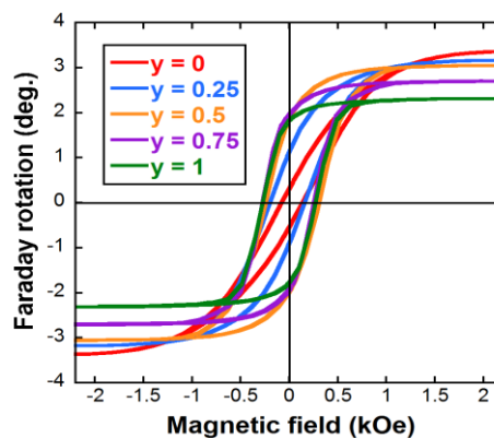
Fig. 1 Faraday hysteresis loops
