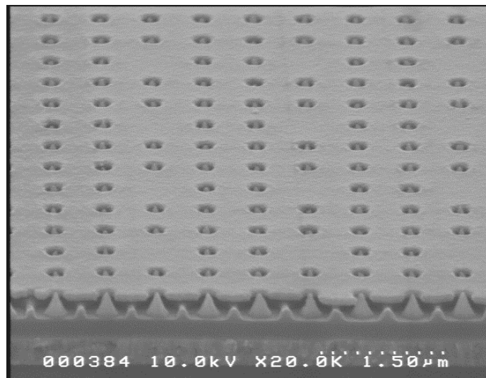
Fig.2 Photograph of Emitter array of the Spindt
