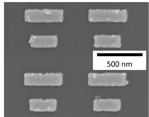
Fig. 1 SEM image of fabricated metamaterial structure
