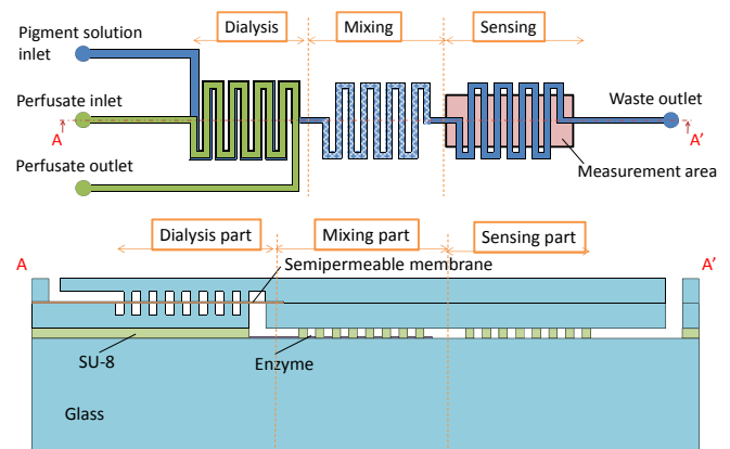
Fig.1 : Schematic view of optical substance concentration sensor.
