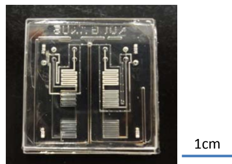
Fig.2 : Fabrication result of flow channel for optical substance concentration sensor.
