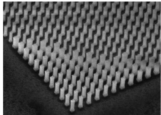
Fig.1 Quasi-two-dimensional periodic fine poly-Si structures fabricated on glass substrate.
