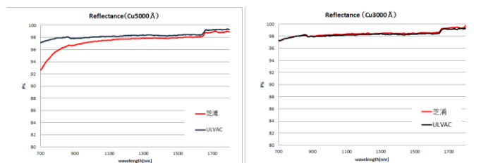
Fig.1 Reflection spectra of different Cu thickness.
